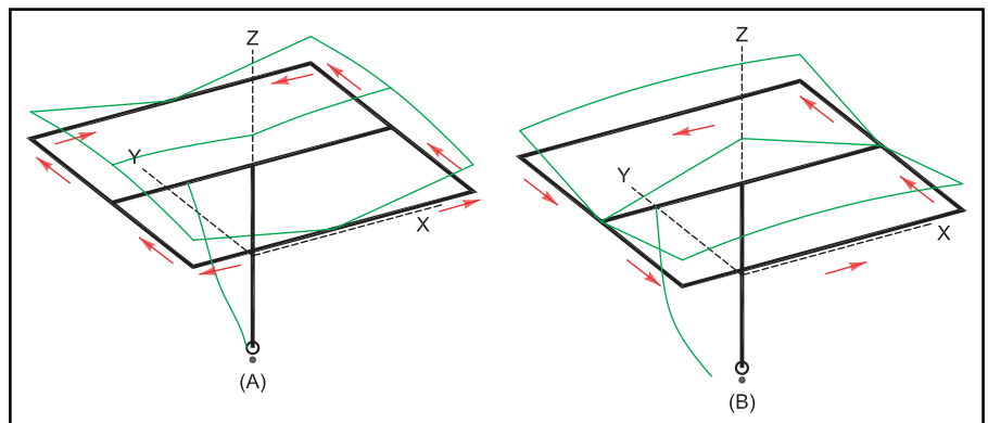
Figure 3—Horizontal quad loops showing currents on the loop wires for the case where the phasing lines provide in-phase feed (A); and out-of-phase feed (B). Note the left phasing line is the transposed feeder. The frequency is 3.75 MHz.
